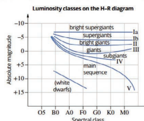
FIGURE 13.2.7 Luminosity class provides an estimation of the vertical position of a star on the H-R diagram when a direct measurement of luminosity is not available.
